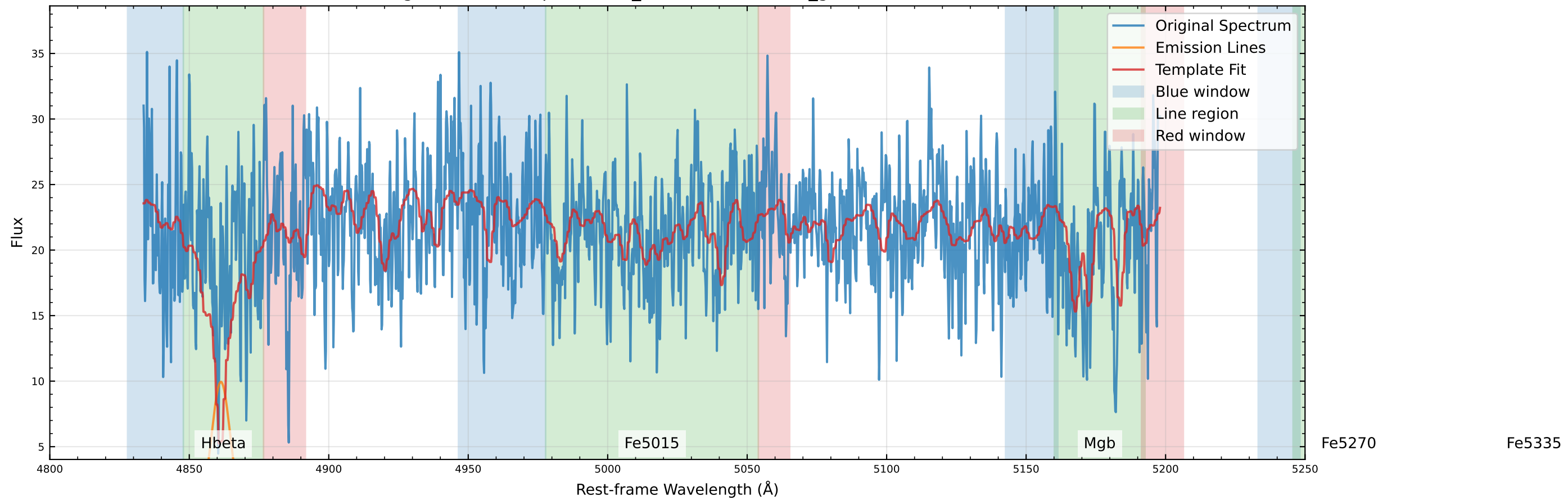
Original Data Comparison (v_star=-97.8 km/s, v_gas=-180.9 km/s)
