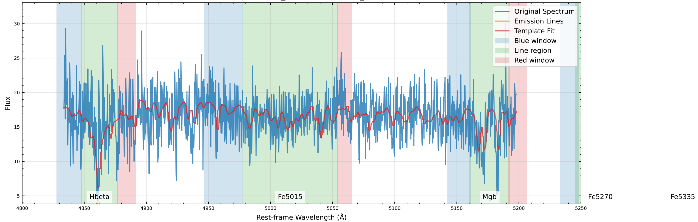
Original Data Comparison (v_star=-60.2 km/s, v_gas=-149.4 km/s)
