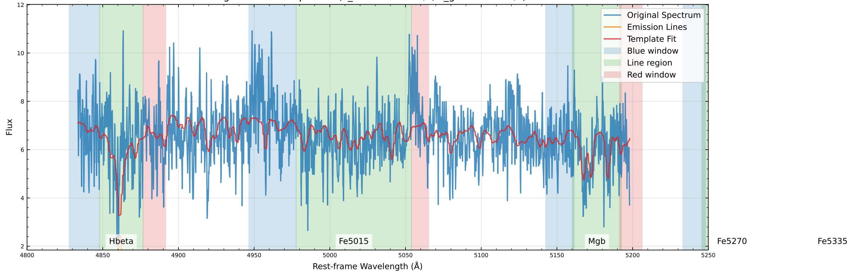
Original Data Comparison (v_star=-33.4 km/s, v_gas=61.8 km/s)
