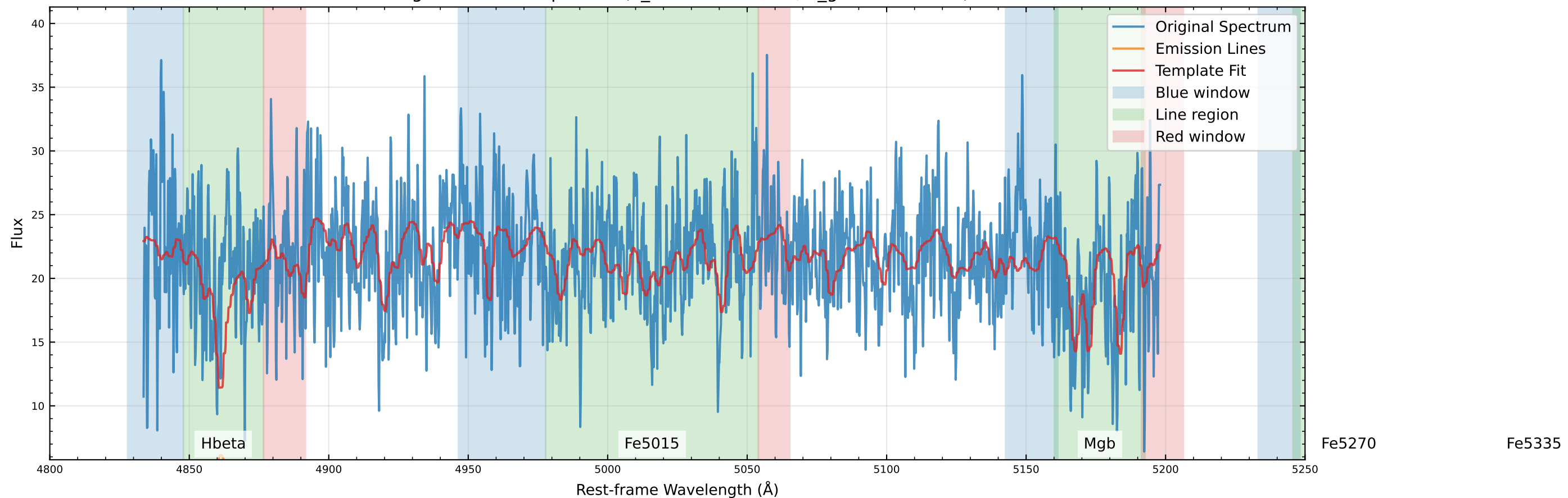
Original Data Comparison (v_star=-60.3 km/s, v_gas=67.4 km/s)
