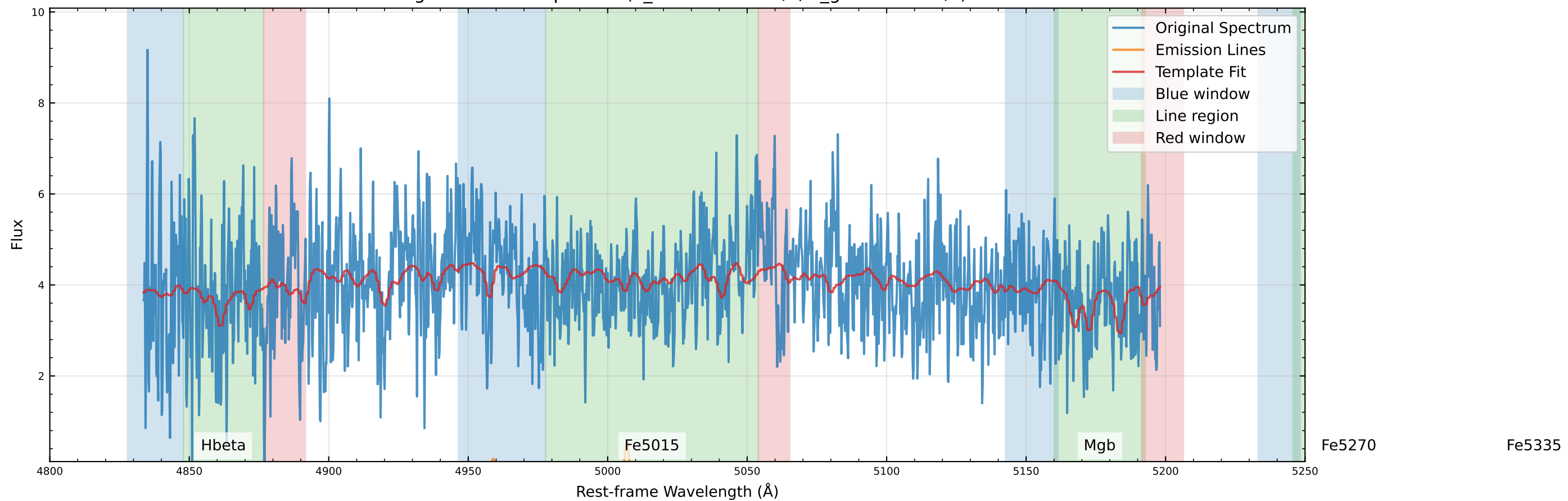
Original Data Comparison (v_star=-48.6 km/s, v_gas=-6.3 km/s)
