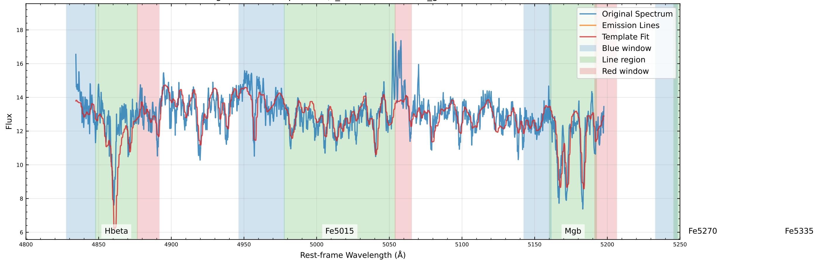
Original Data Comparison ( v_{\text{star}}=-42.2 km/s, v_{\text{gas}}=-3.6 km/s)
