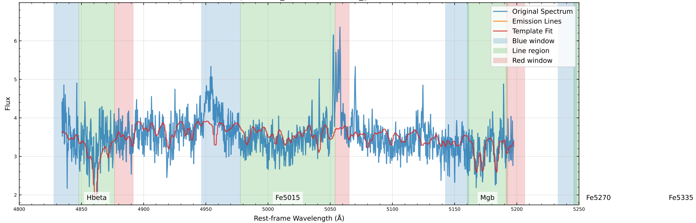
Original Data Comparison (v_star=-43.2 km/s, v_gas=195.3 km/s)
