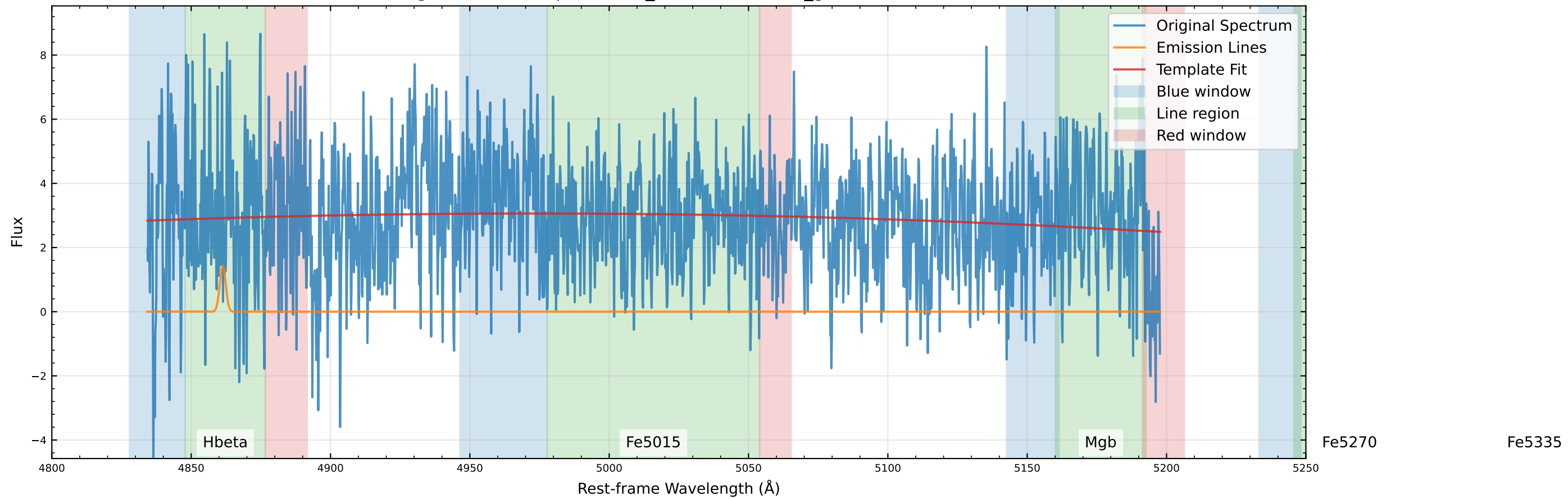
Original Data Comparison (v_star=0.0 km/s, v_gas=134.5 km/s)
