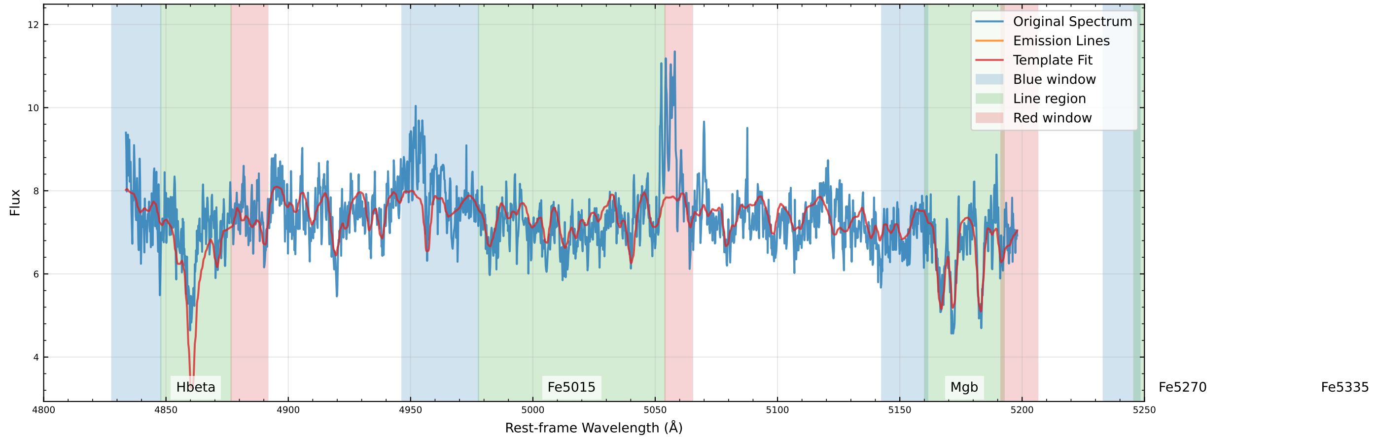
Original Data Comparison (v_star=-40.1 km/s, v_gas=25.6 km/s)
