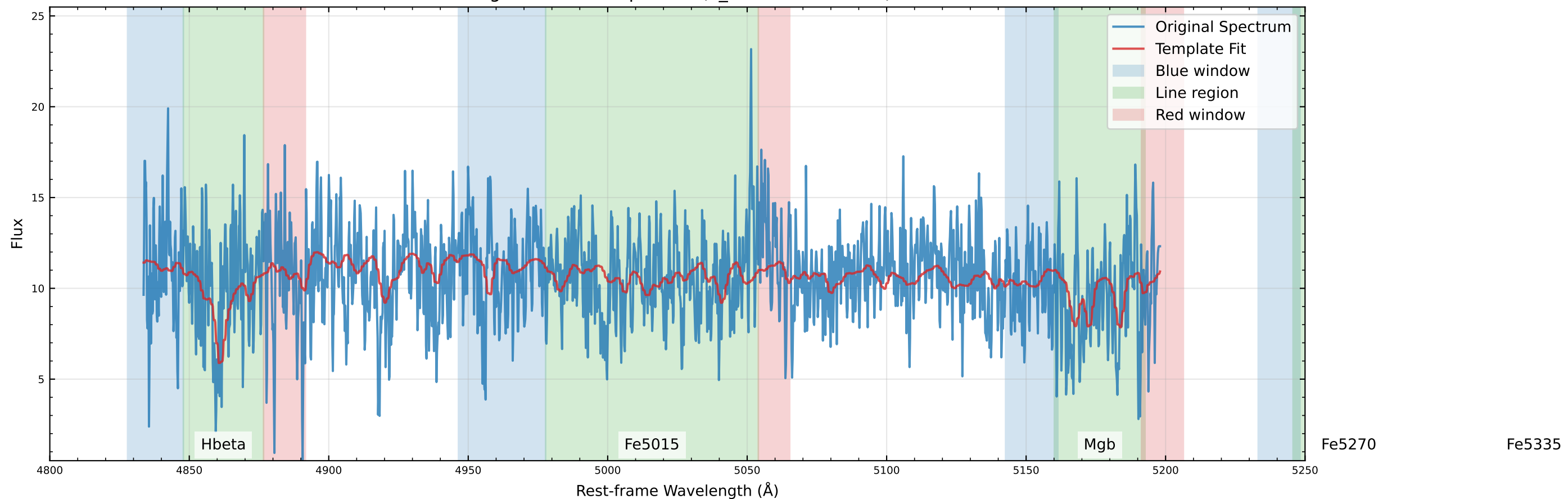
Original Data Comparison (v_star=-101.2 km/s)
