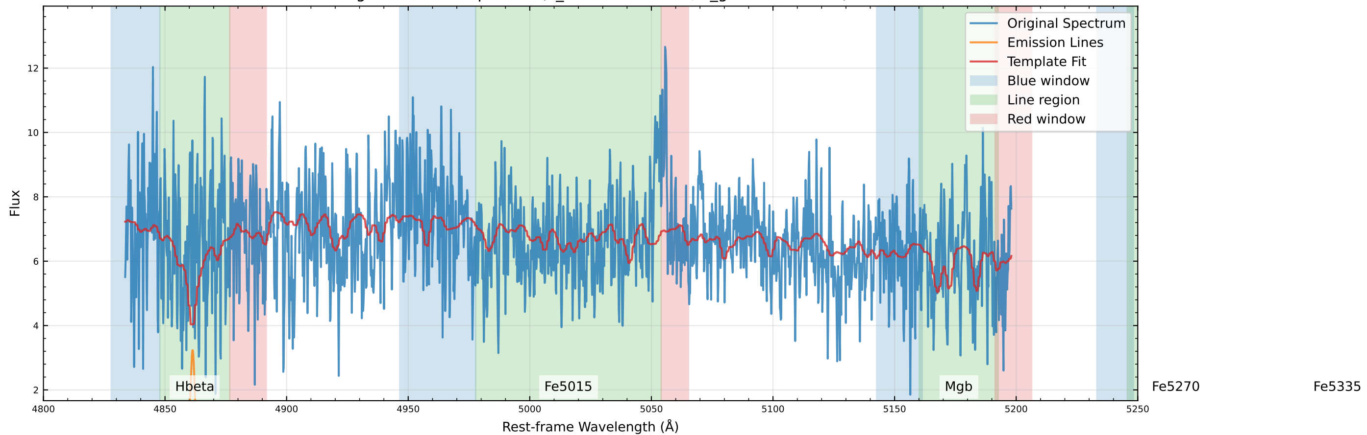
Original Data Comparison ( v_{\text{star}}=-93.4 km/s, v_{\text{gas}}=-65.7 km/s)
