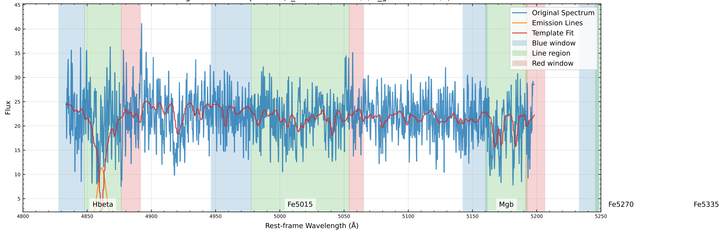
Original Data Comparison (v_star=-102.4 km/s, v_gas=-90.1 km/s)
