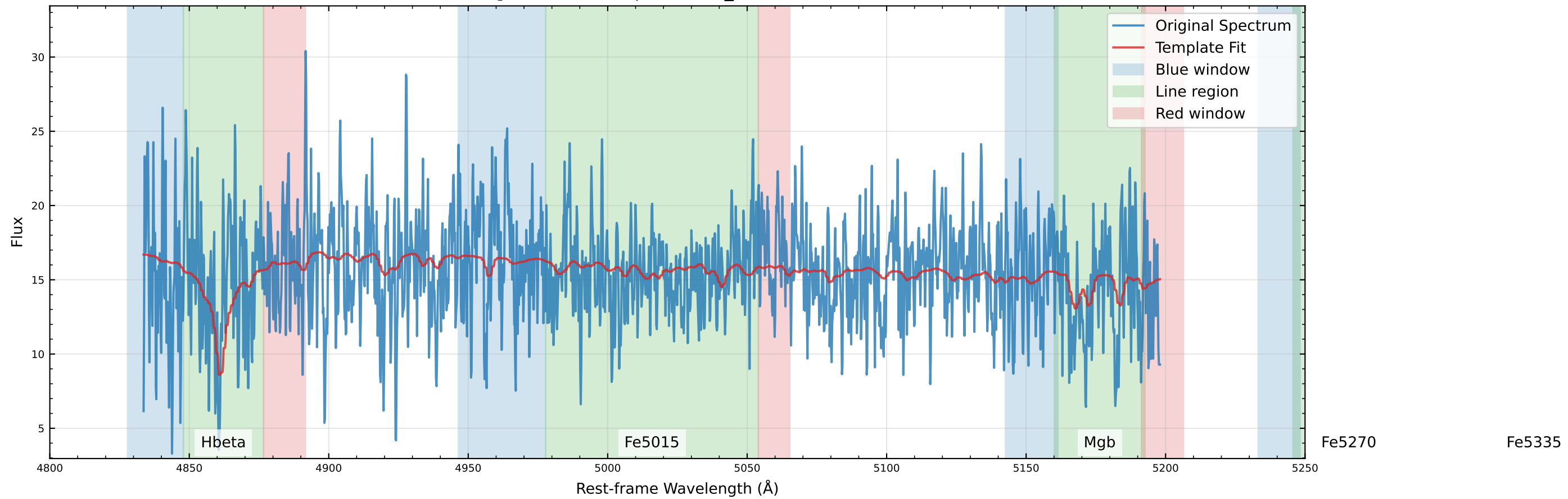
Original Data Comparison (v_star=-70.3 km/s)
