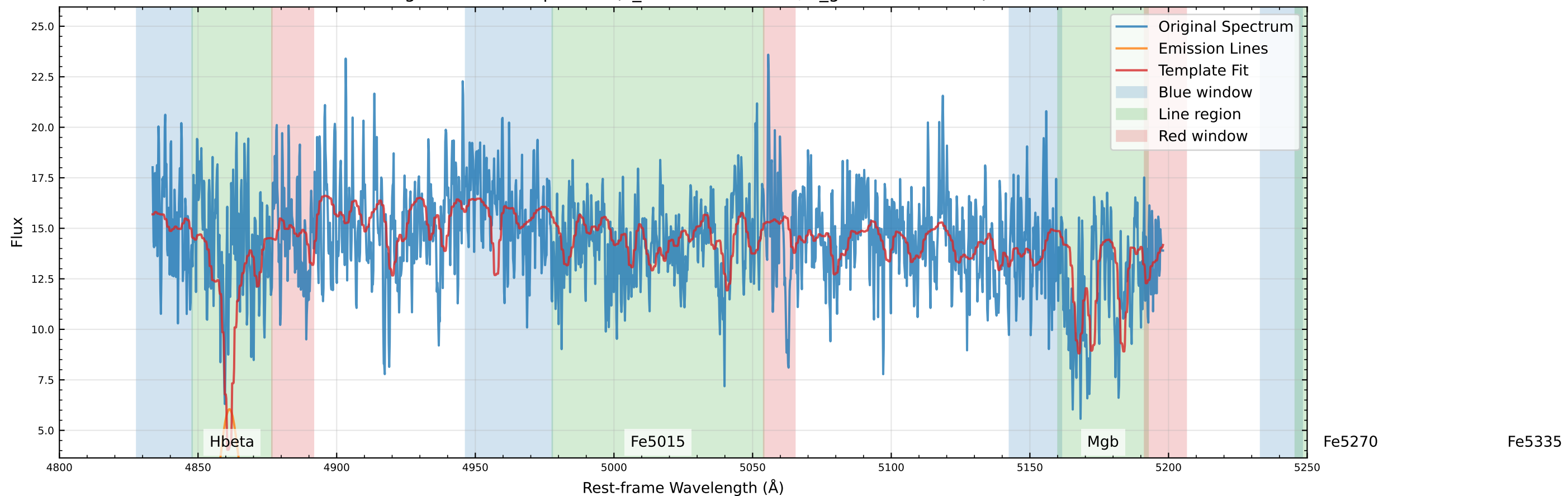
Original Data Comparison (v_star=-122.2 km/s, v_gas=-137.9 km/s)
