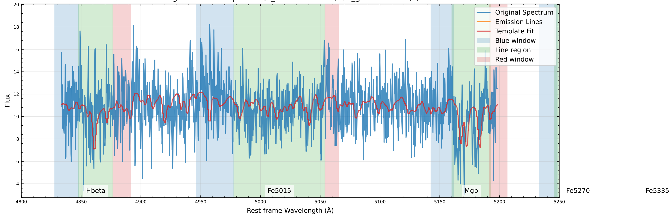
Original Data Comparison (v_star=-118.2 km/s, v_gas=-24.3 km/s)
