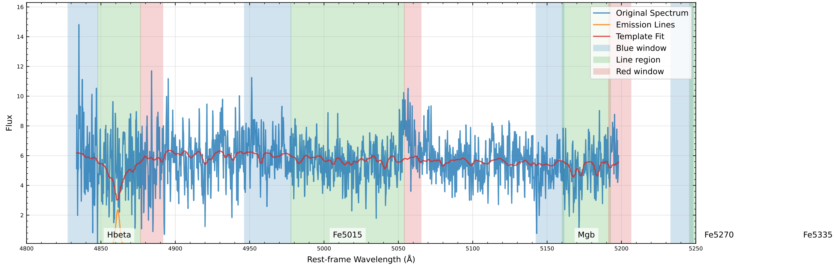
Original Data Comparison ( v_{\text{star}}=-11.8 km/s, v_{\text{gas}}=-38.8 km/s)
