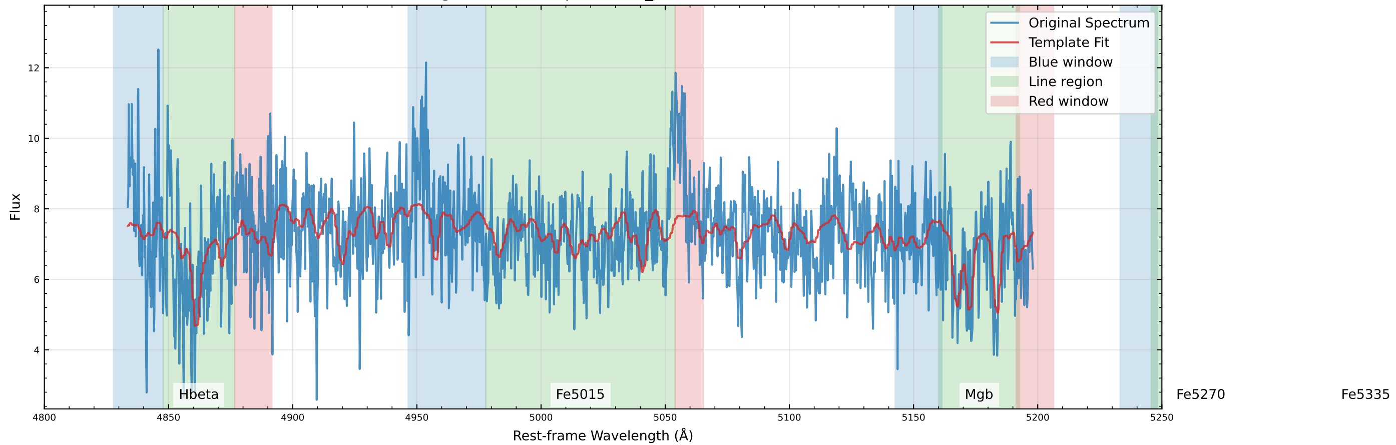
Original Data Comparison (v_star=-28.5 km/s)
