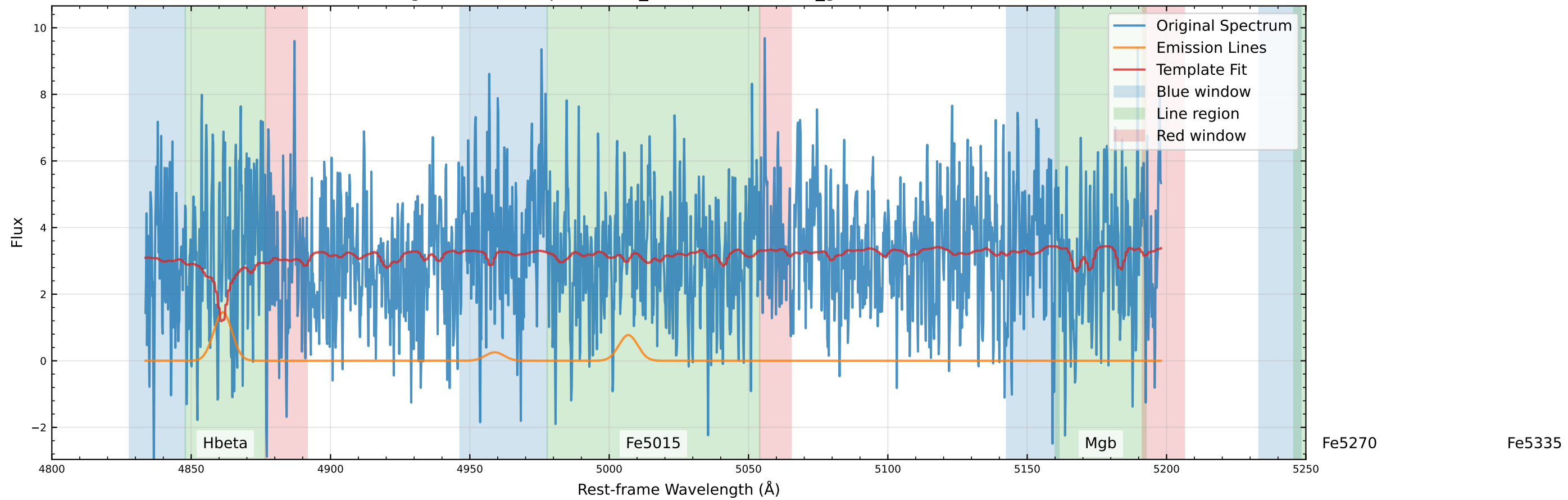
Original Data Comparison (v_star=-79.1 km/s, v_gas=-70.6 km/s)
