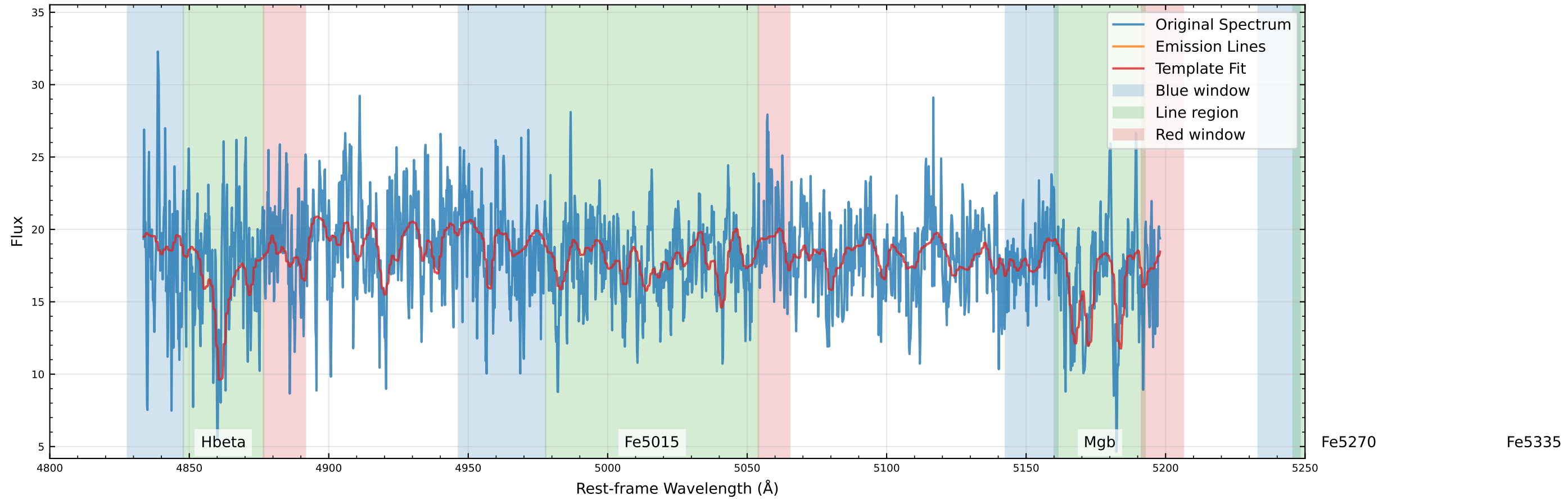
Original Data Comparison (v_star=-51.4 km/s, v_gas=65.3 km/s)
