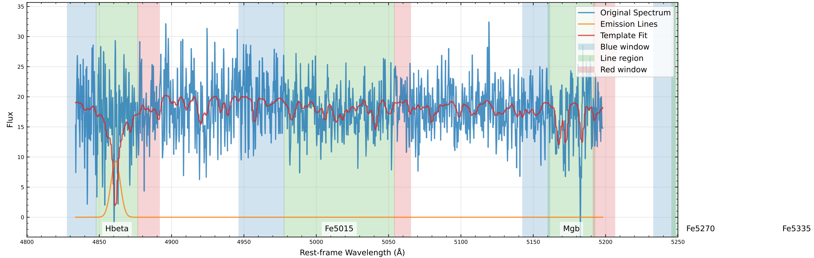
Original Data Comparison (v_star=-58.1 km/s, v_gas=-68.6 km/s)
