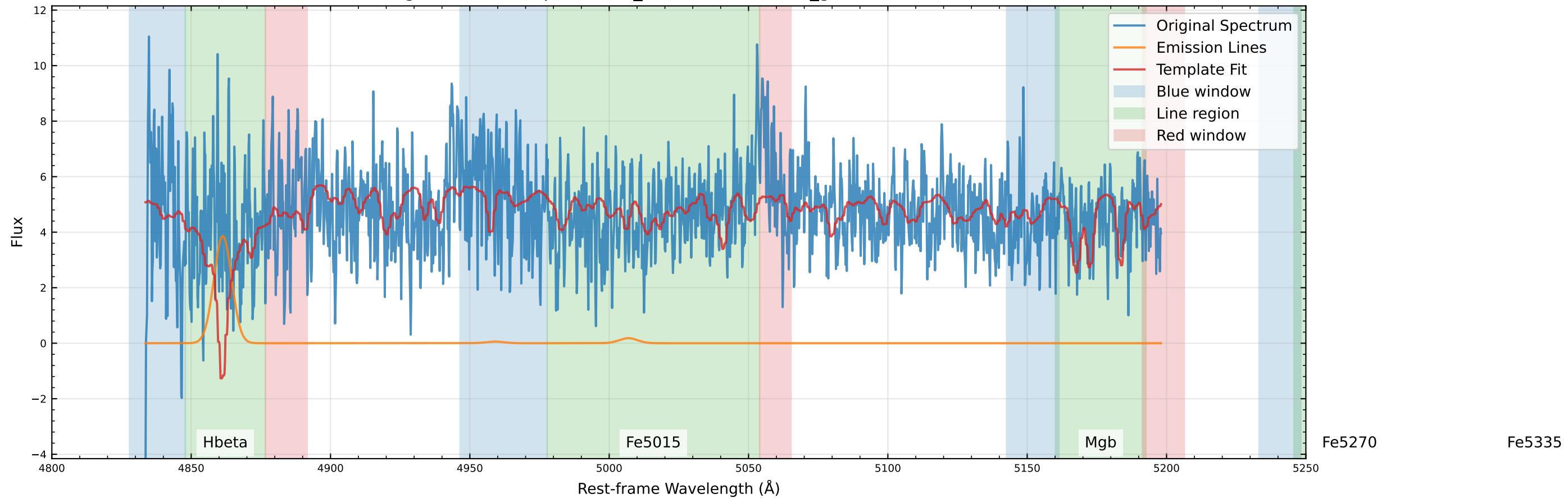
Original Data Comparison (v_star=-53.7 km/s, v_gas=-149.2 km/s)
