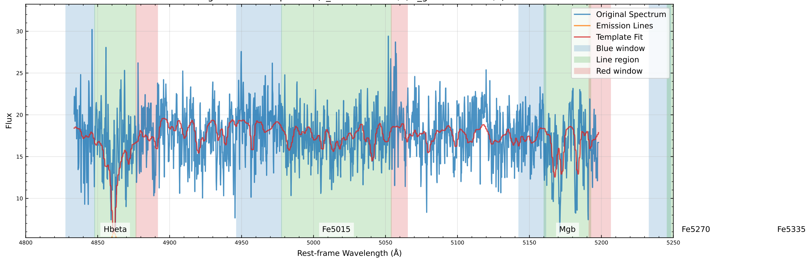
Original Data Comparison (v_star=-75.4 km/s, v_gas=-116.5 km/s)
