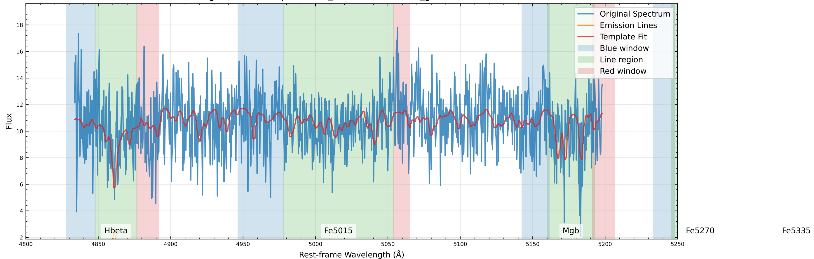
Original Data Comparison (v_star=-69.8 km/s, v_gas=-134.8 km/s)
