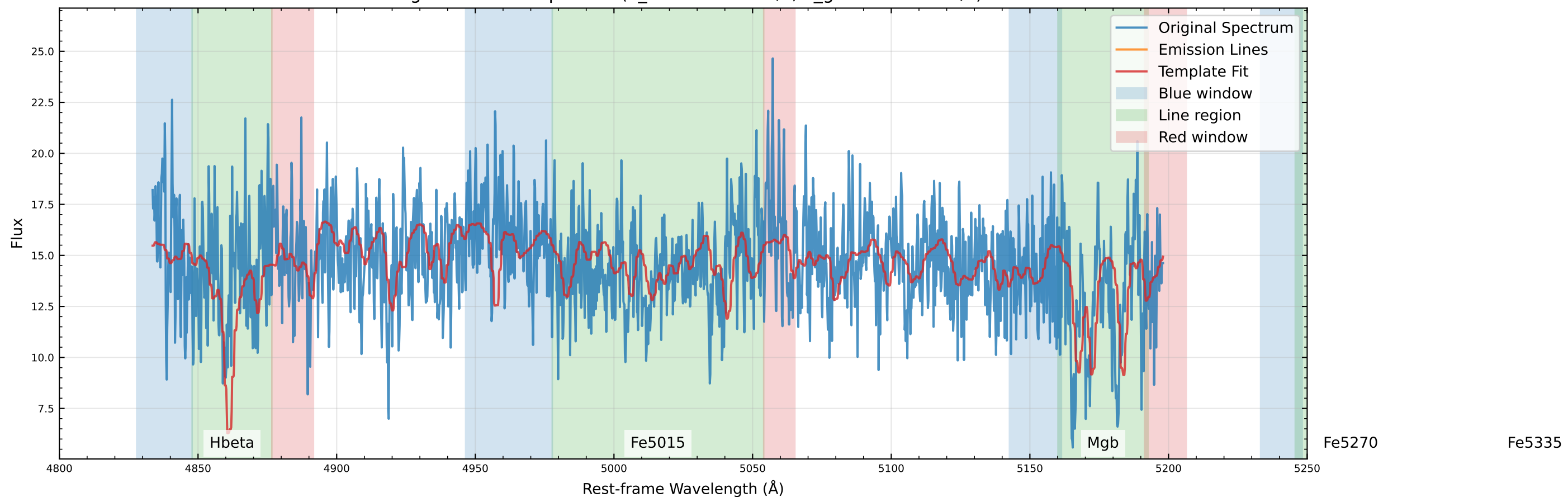
Original Data Comparison (v_star=-99.8 km/s, v_gas=-102.3 km/s)
