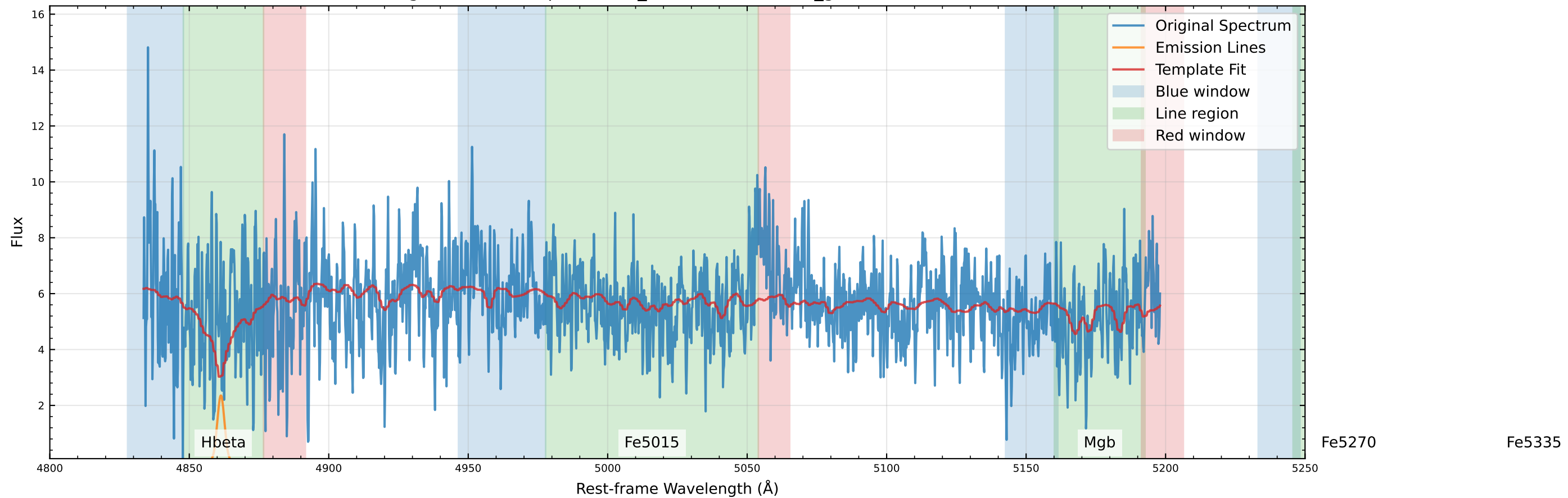
Original Data Comparison (v_star=-11.8 km/s, v_gas=-38.8 km/s)
