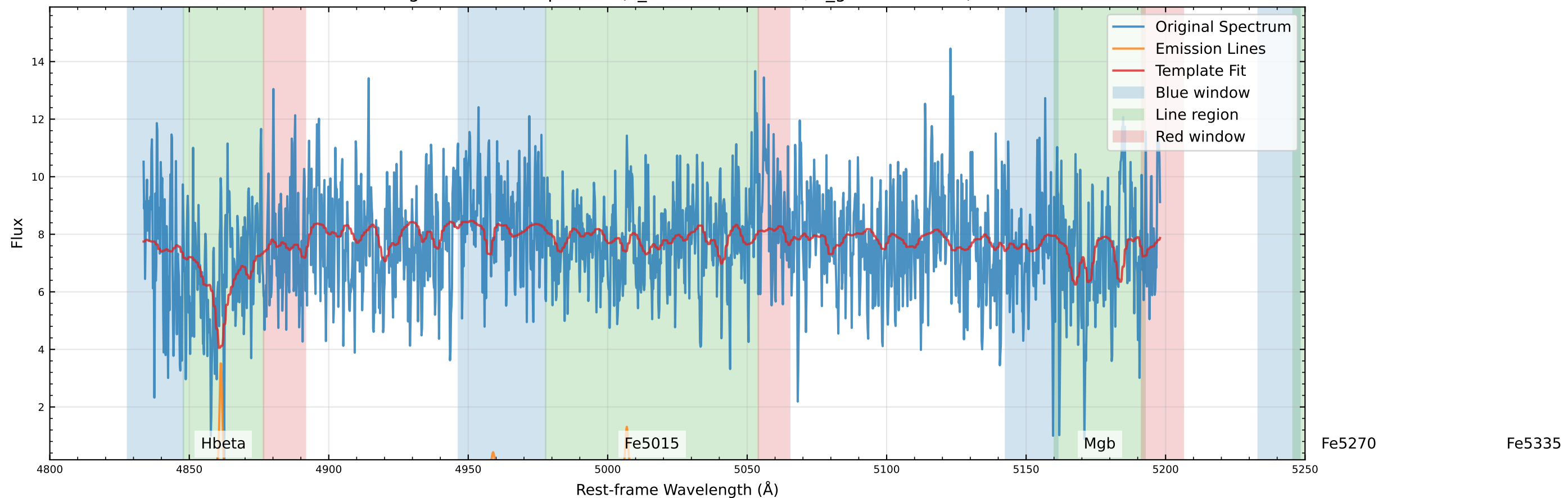
Original Data Comparison (v_star=-114.0 km/s, v_gas=-4.4 km/s)
