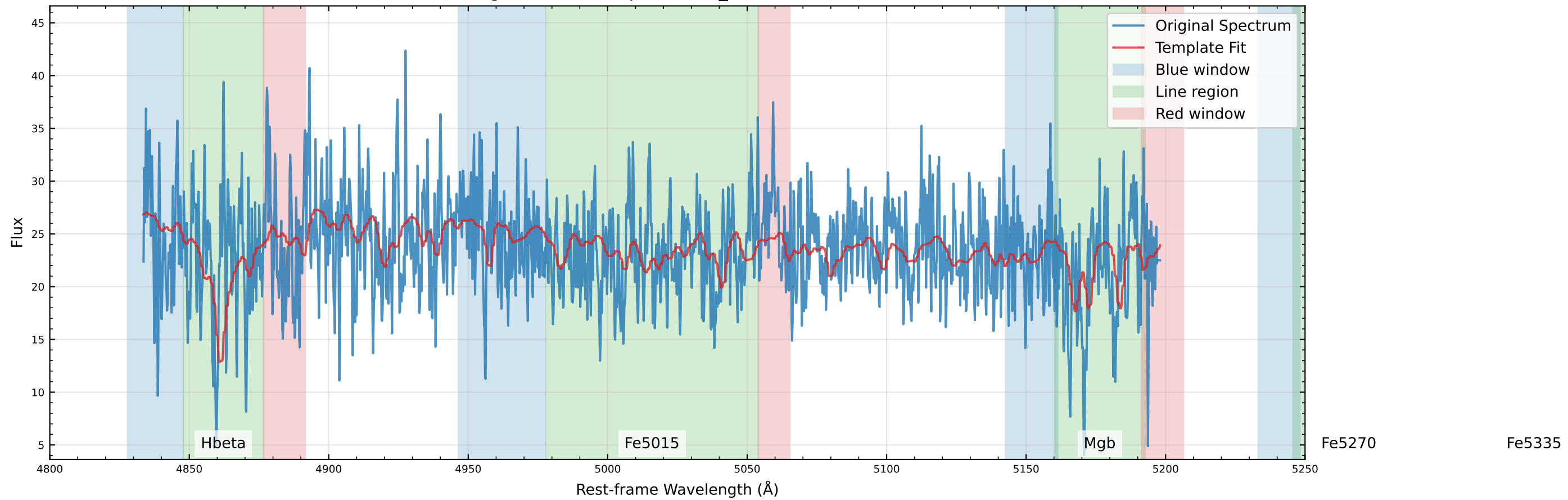
Original Data Comparison (v_star=-116.4 km/s)
