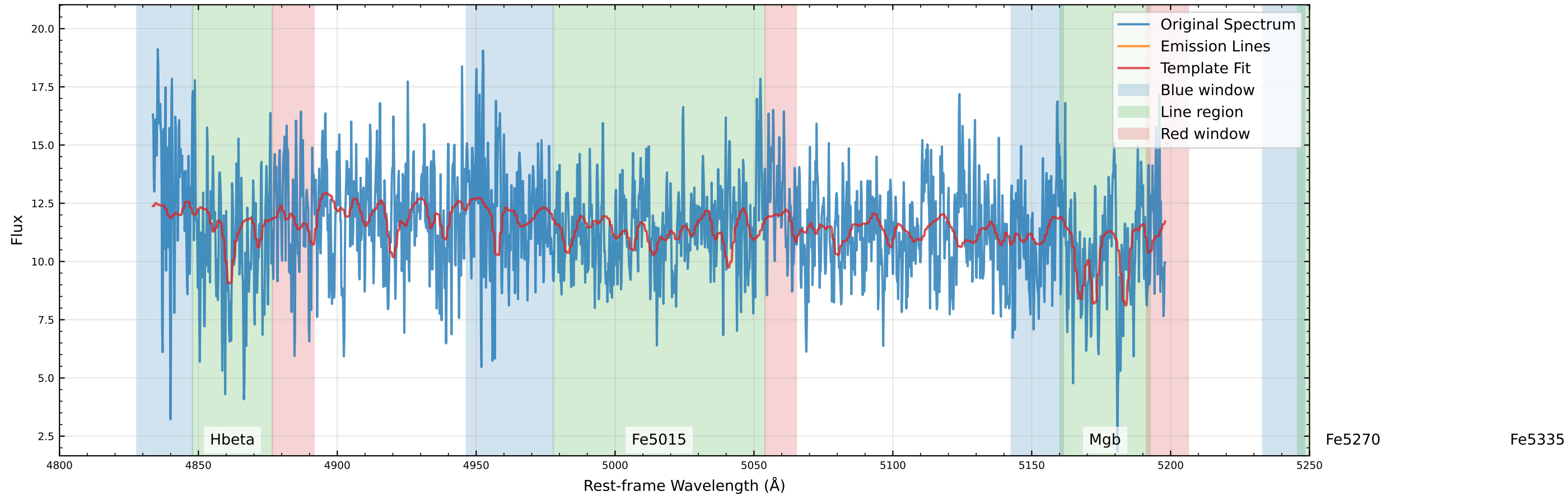
Original Data Comparison (v_star=-106.0 km/s, v_gas=194.0 km/s)
