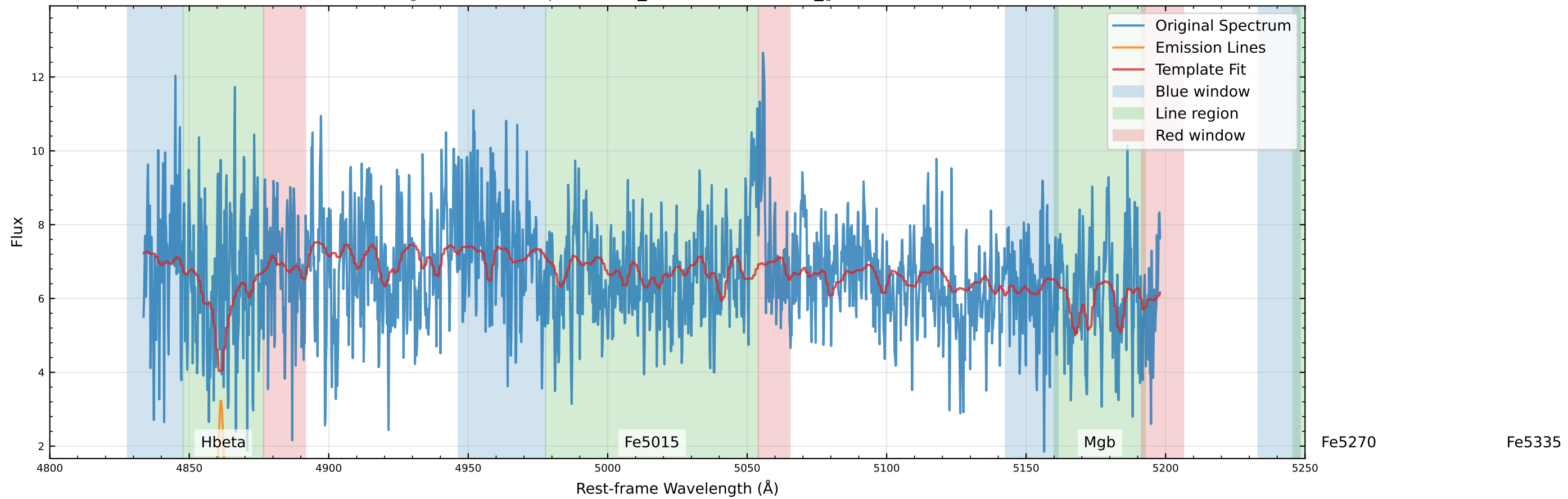
Original Data Comparison (v_star=-93.4 km/s, v_gas=-65.7 km/s)
