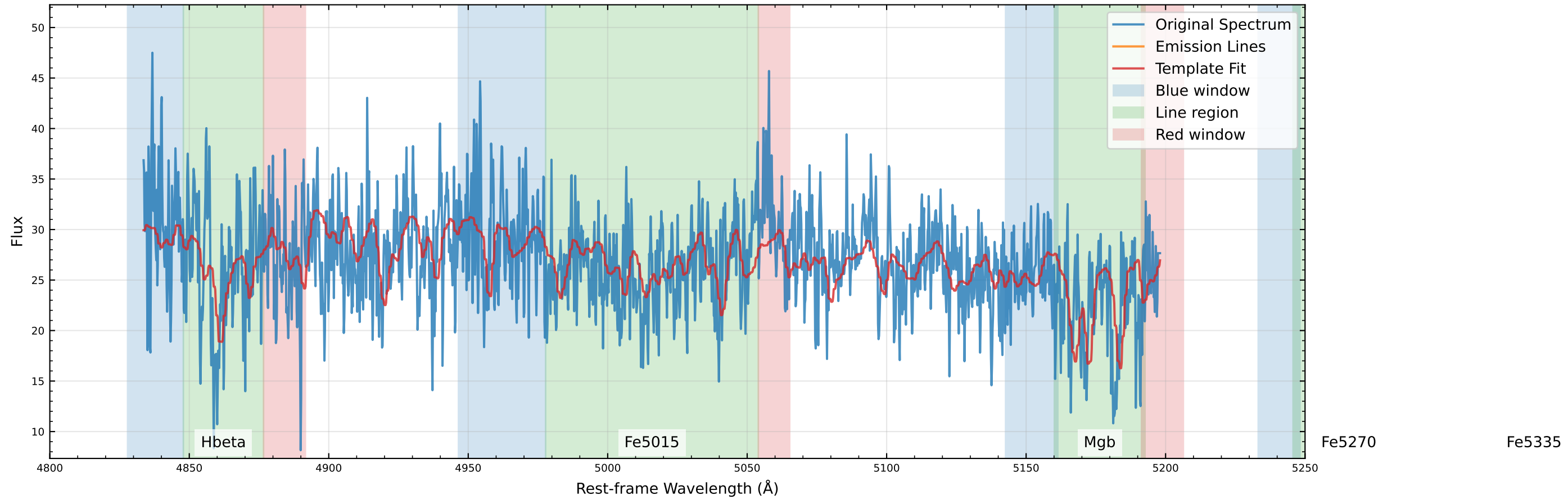
Original Data Comparison (v_star=-93.2 km/s, v_gas=-13.4 km/s)
