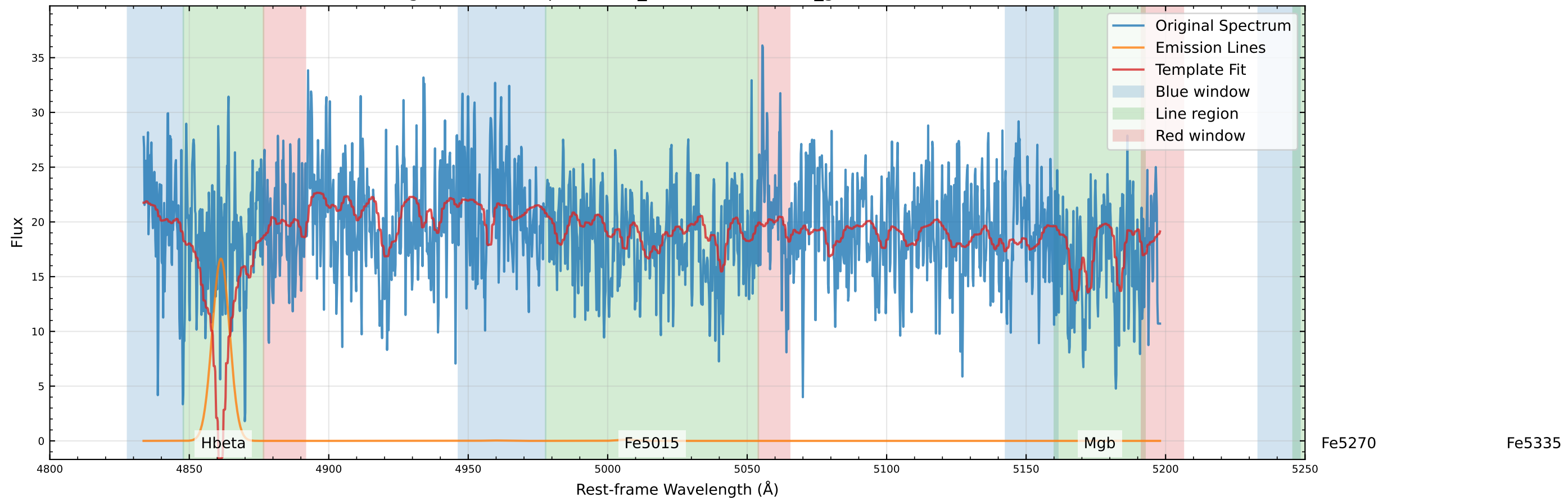
Original Data Comparison (v_star=-93.7 km/s, v_gas=-85.5 km/s)
