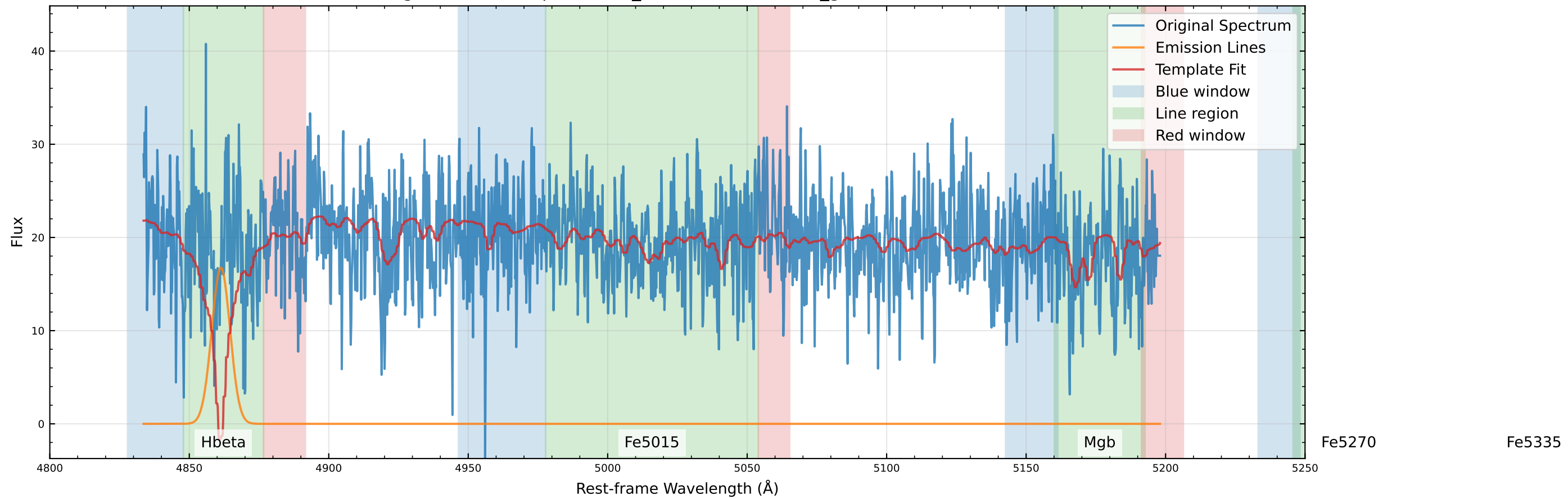
Original Data Comparison (v_star=-109.7 km/s, v_gas=-86.7 km/s)
