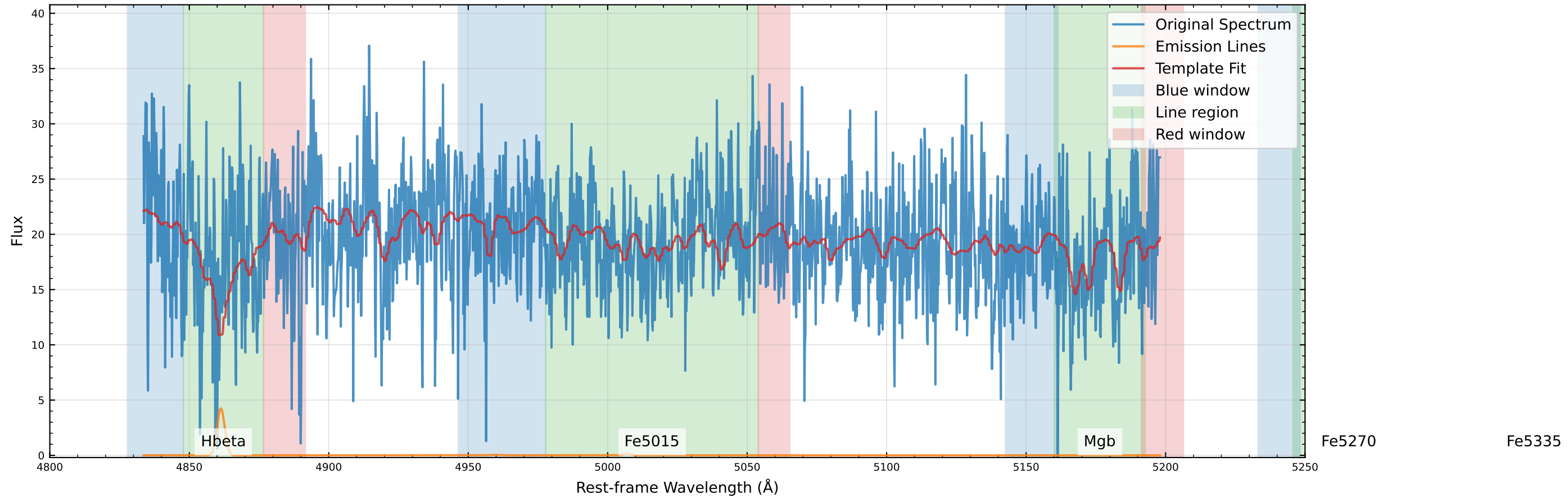
Original Data Comparison (v_star=-63.5 km/s, v_gas=-246.4 km/s)
