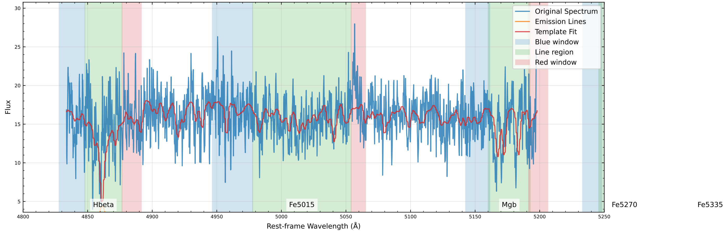
Original Data Comparison (v_star=-85.1 km/s, v_gas=22.8 km/s)
