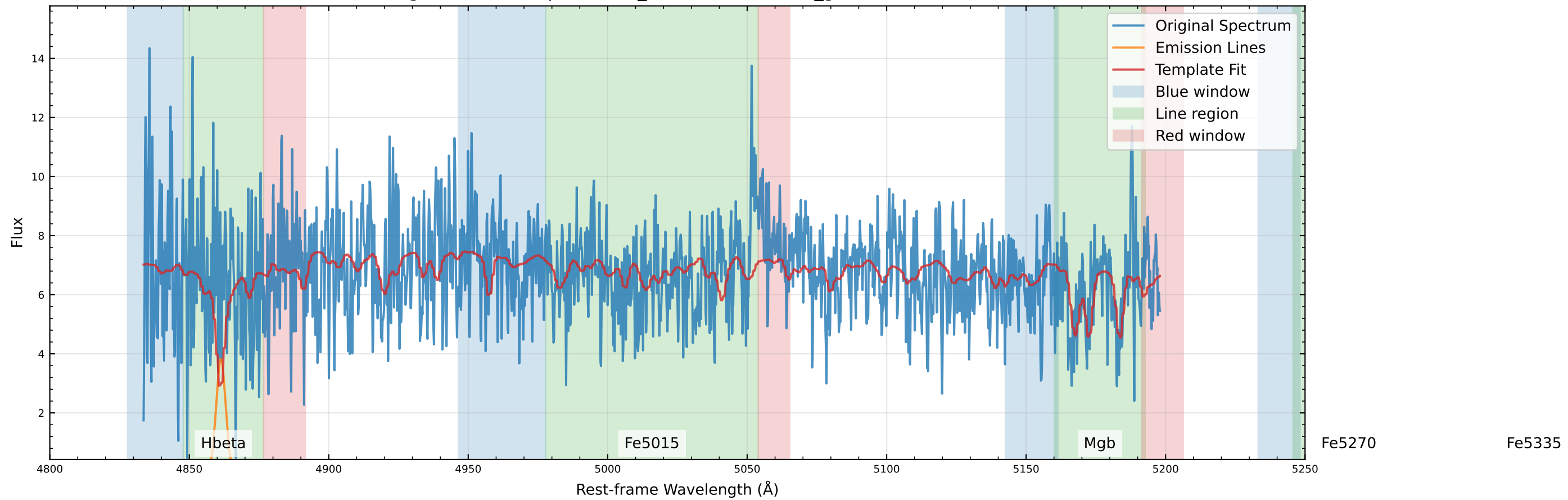
Original Data Comparison (v_star=-53.4 km/s, v_gas=-71.9 km/s)
