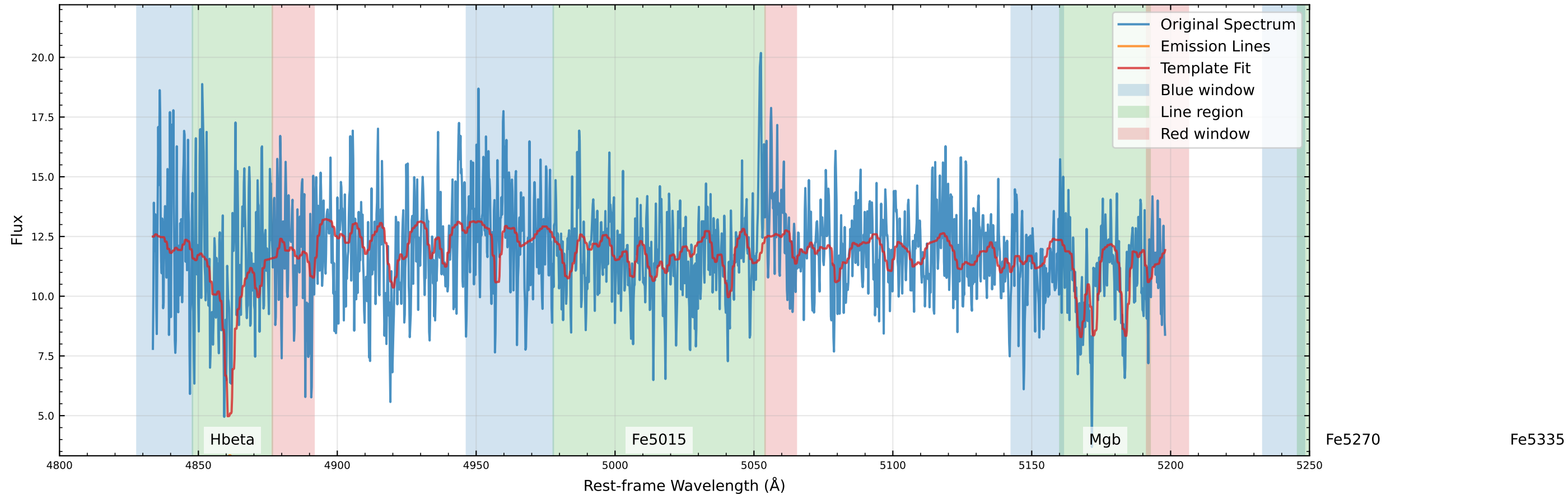
Original Data Comparison (v_star=-39.8 km/s, v_gas=53.2 km/s)
