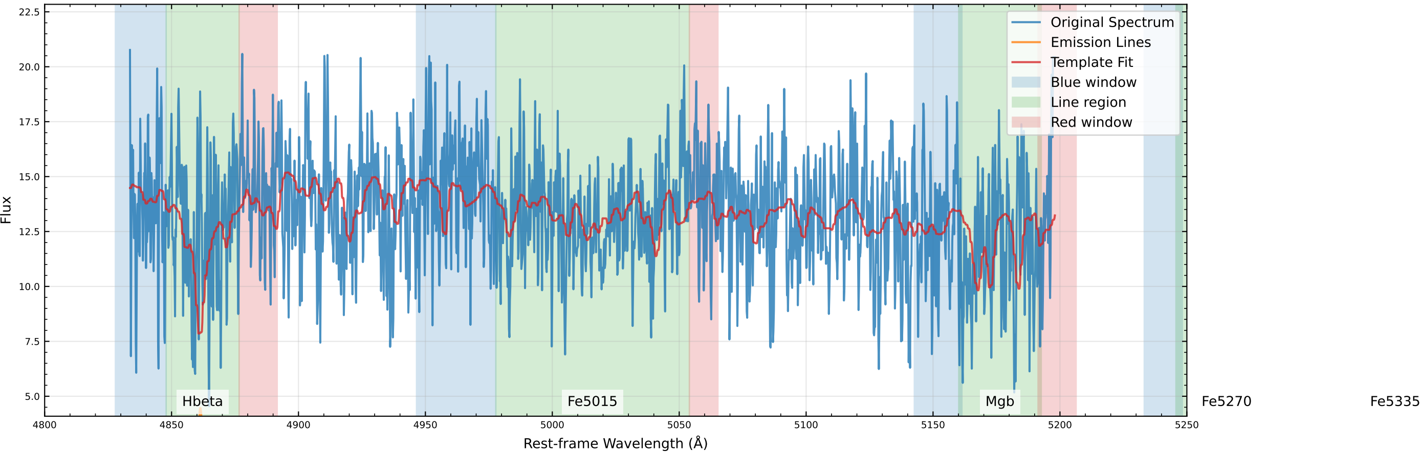
Original Data Comparison (v_star=-140.2 km/s, v_gas=-42.2 km/s)
