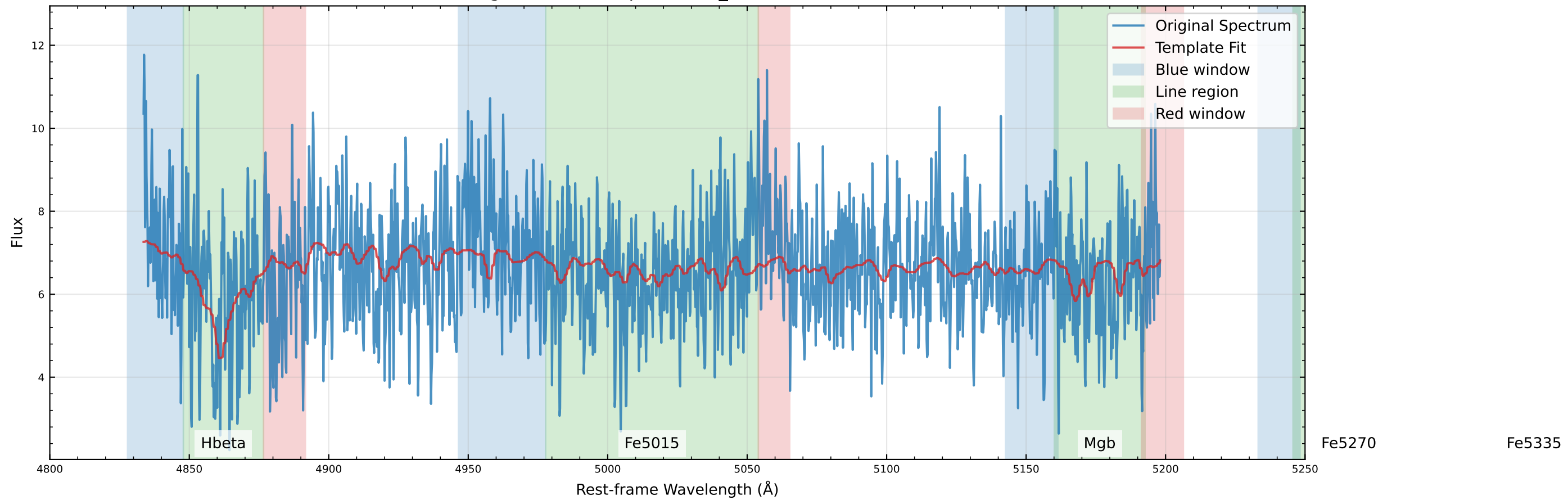
Original Data Comparison (v_star=-150.1 km/s)
