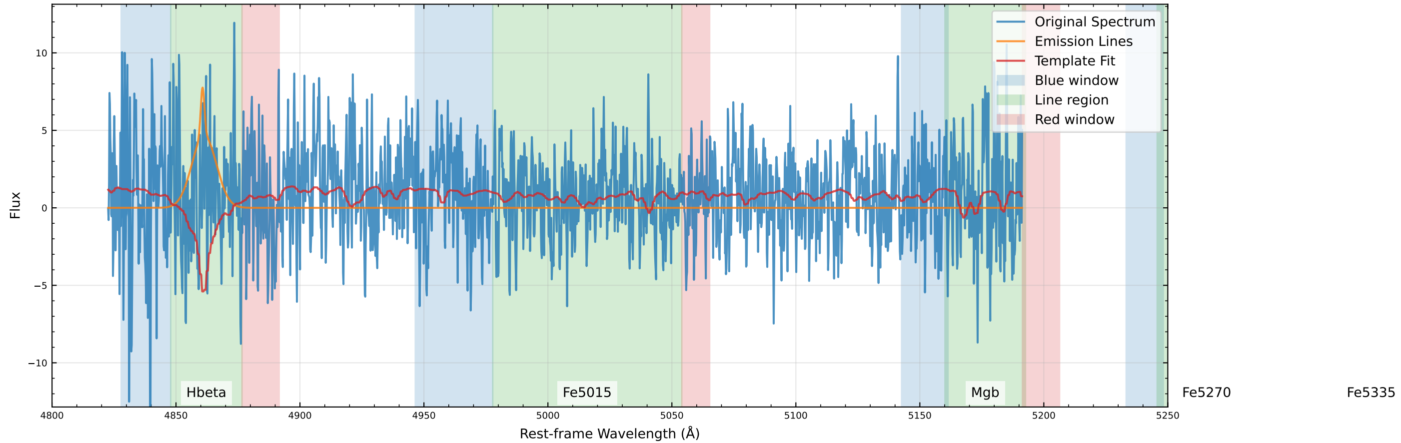
Original Data Comparison (v_star=332.2 km/s, v_gas=333.8 km/s)
