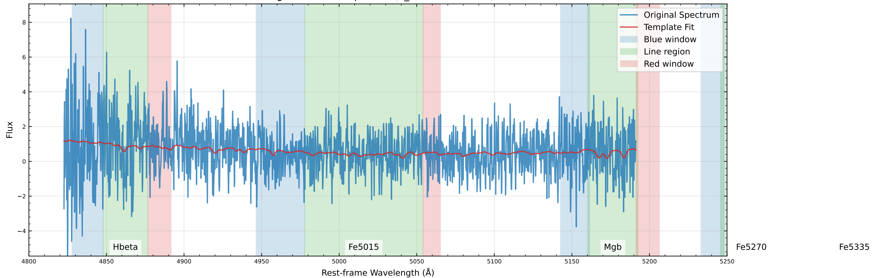
Original Data Comparison (v_star=-39.0 km/s)
