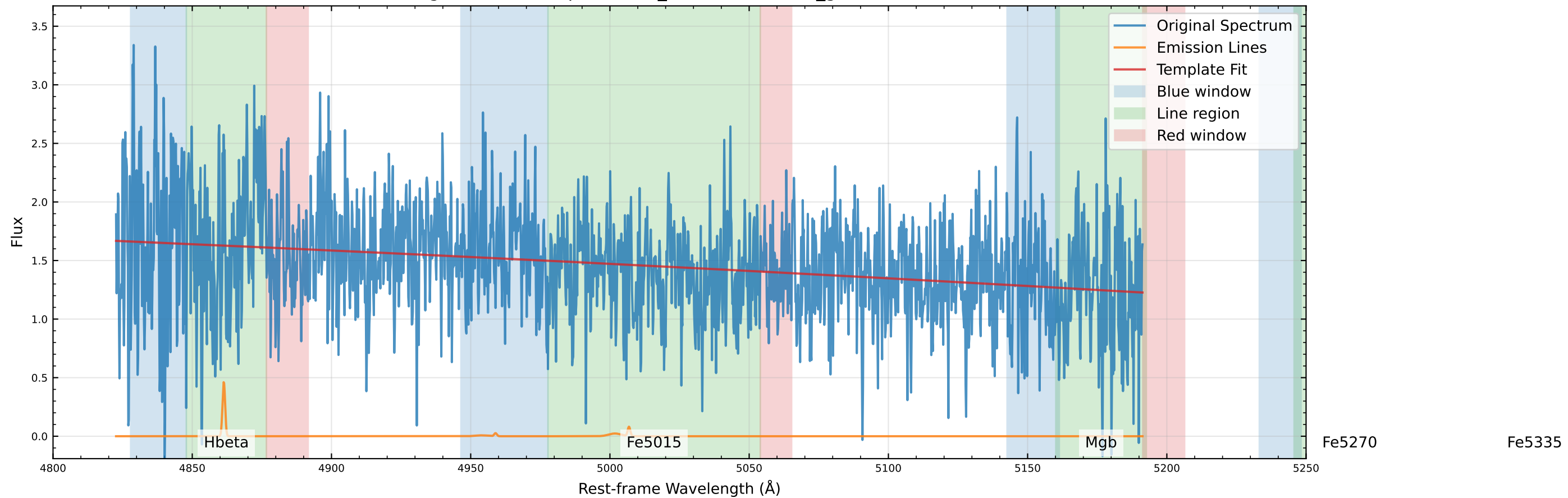
Original Data Comparison (v_star=0.0 km/s, v_gas=2.9 km/s)
