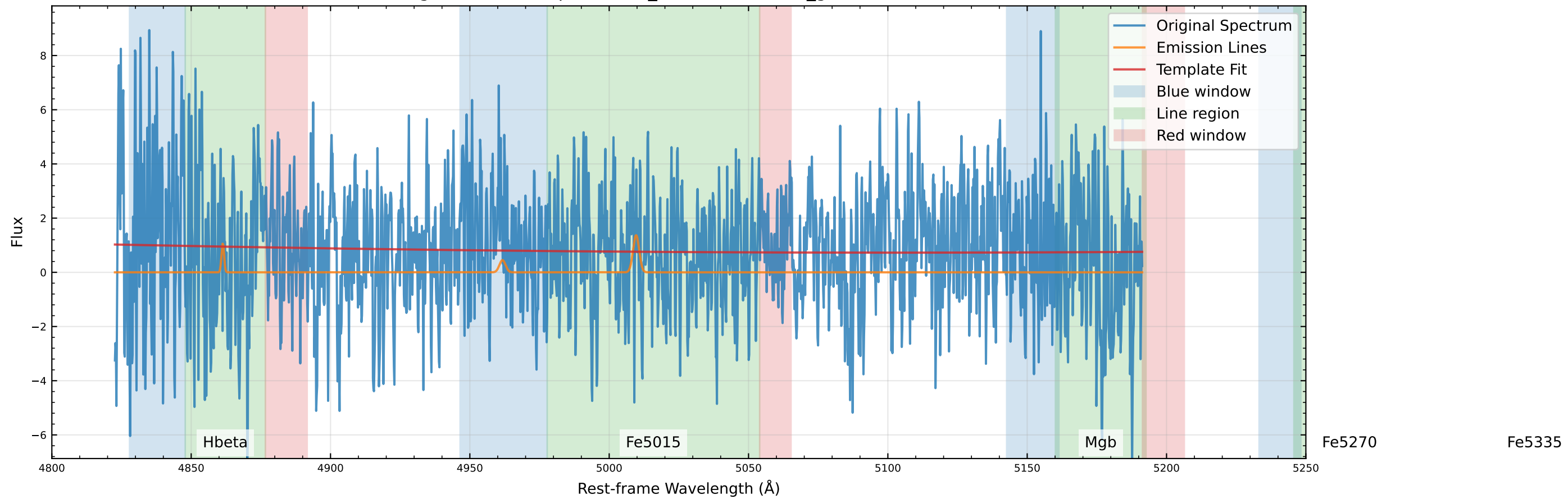
Original Data Comparison (v_star=0.0 km/s, v_gas=-58.0 km/s)
