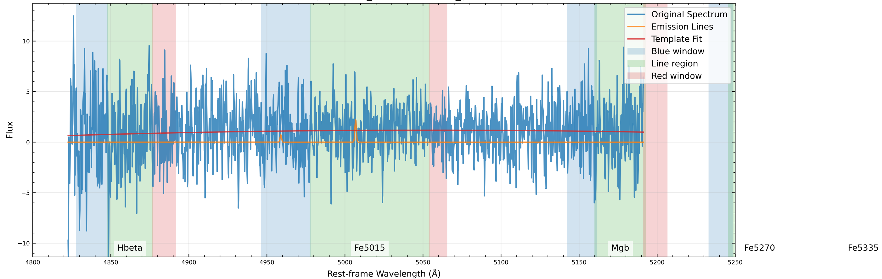
Original Data Comparison (v_star=0.0 km/s, v_gas=-18.0 km/s)
