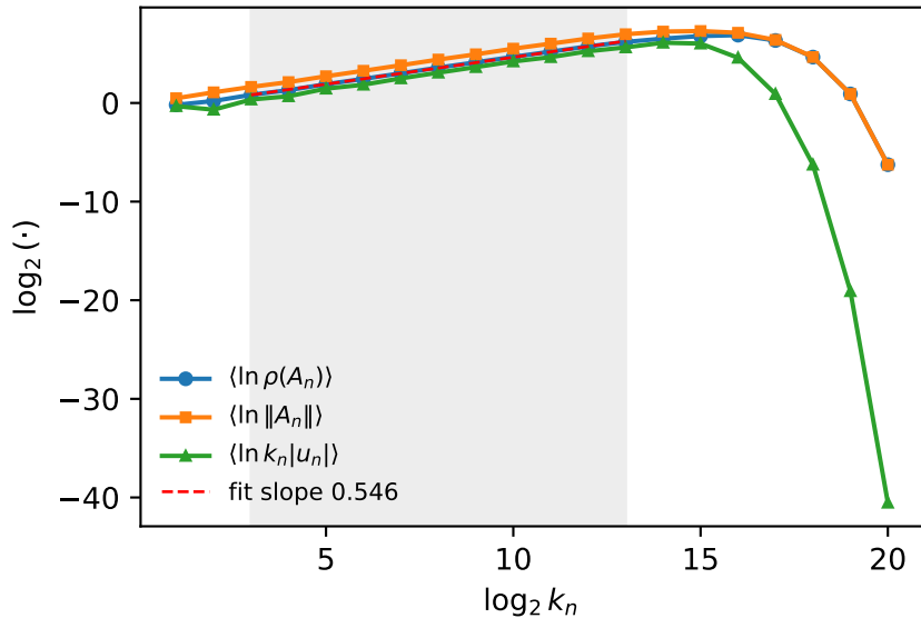
(b) cascade scaling ( r = 1 )
