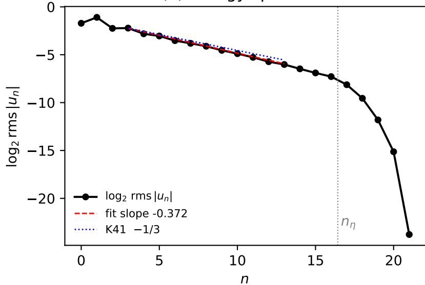
(a) energy spectrum
