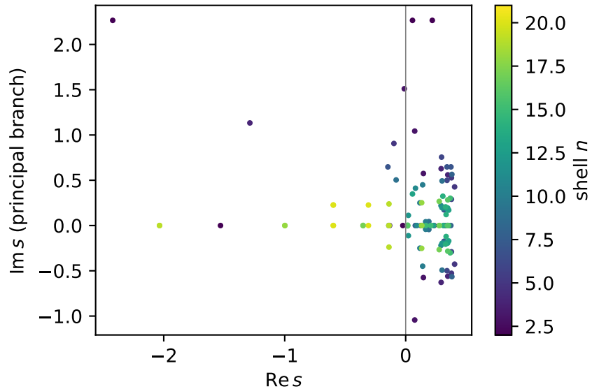
(a) dynamical poles of \Lambda_u(\cdot, t) , one snapshot
