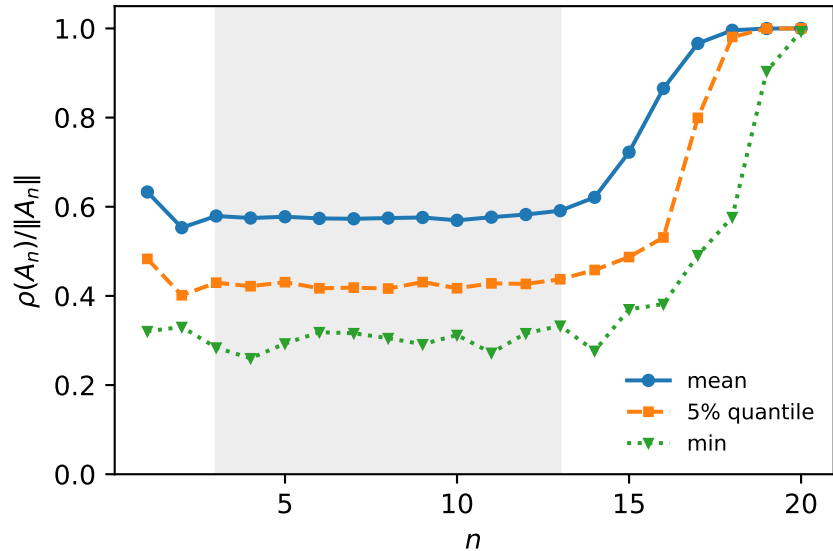
(a) non-normality is bounded
