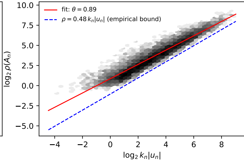
(b) spectral lower bound (inertial range)
