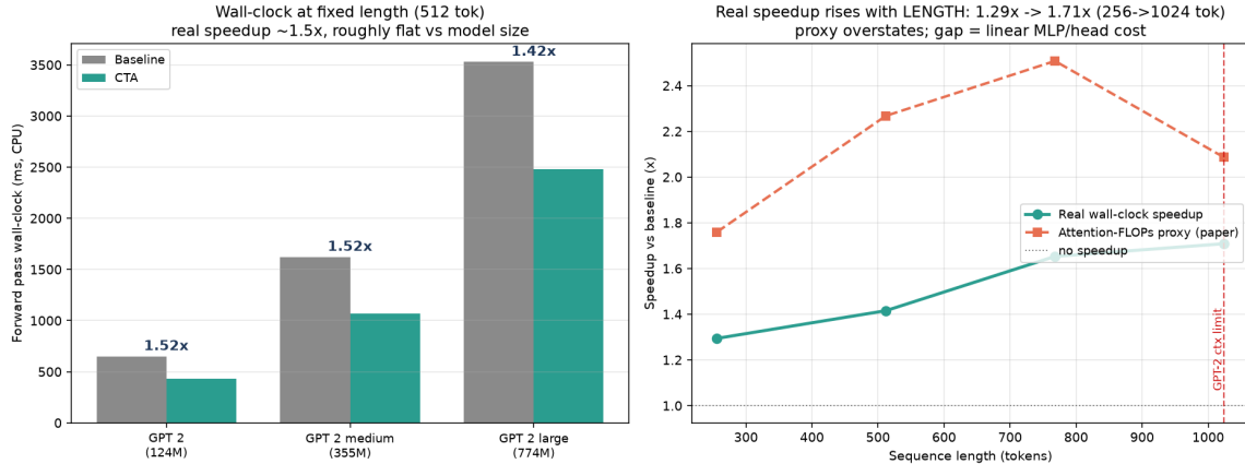
Figure 3: Left: realized wall-clock (baseline vs. CTA) at 512 tokens across the GPT-2 size ladder; the speedup is \sim 1.5\times and roughly flat in model size. Right: realized speedup vs. sequence length on GPT-2 small, against the attention-FLOPs proxy. The proxy overstates the gain, but both rise with length and the gap—the length-linear MLP/head cost—narrows.
