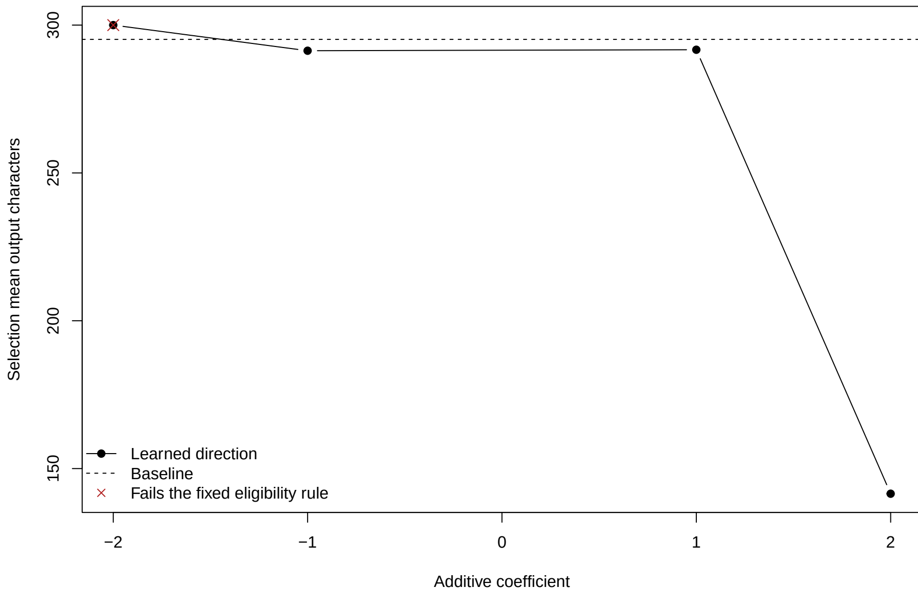
Fixed coefficient grid on six selection tasks
