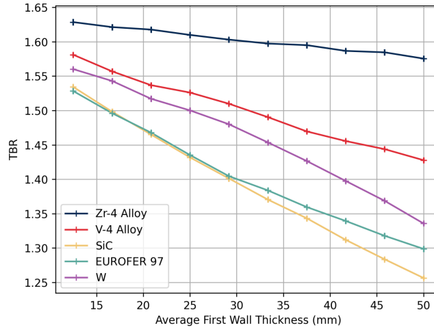
Figure 9: TBR degradation as a function of First Wall (FW) thickness for various candidate materials, including EUROFER97 [50] and Zr-4 as defined in Section 4.3.2. Zirconium-based alloys demonstrate the lowest parasitic absorption, maintaining the highest TBR profile. Error bars are included but are too small to be visible at this scale.
