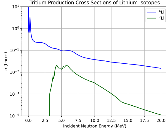
Figure 2: Neutron cross-sections for the primary tritium breeding reactions, {}^6\text{Li}(\text{n},\alpha)\text{t} and {}^7\text{Li}(\text{n}, \text{n}'\alpha)\text{t} , as a function of incident neutron energy. Note the dominance of {}^6\text{Li} at thermal energies.
