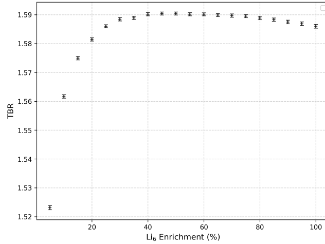
Figure 5: Tritium Breeding Ratio (TBR) as a function of 6 Li enrichment percentage. The curve is characterised by a rapid initial increase which saturates early; the “knee” of the curve appears at approximately 20%, with the TBR effectively capping at 40%. Beyond this saturation point, the returns are diminishing. Notably, a slight suppression in breeding performance is observed at near-total enrichment levels (> 90%)
